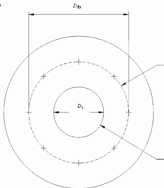
Figure 6.1 Bolted flanged connections
