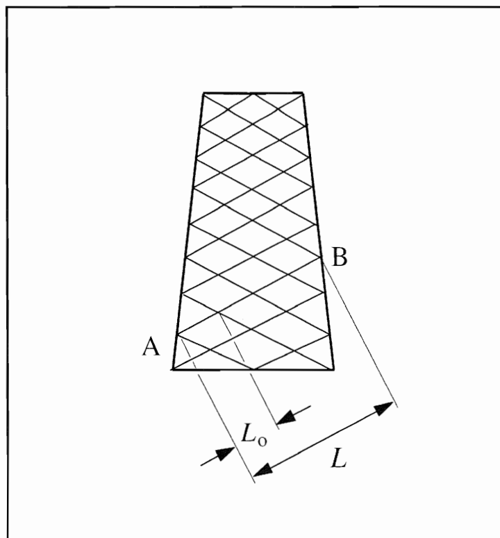
Figure H.7 Multiple lattice bracing
