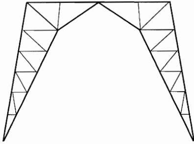
Figure H.5 Cranked K bracing
