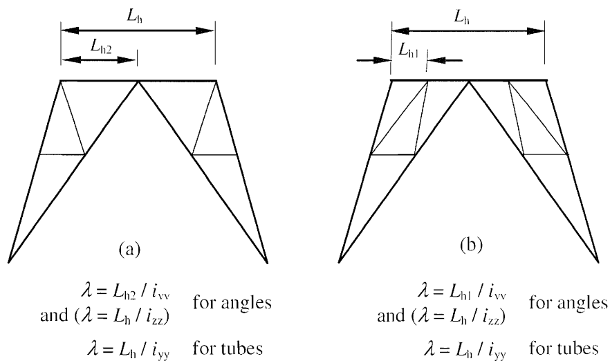
Figure H.4 K bracing horizontals without plan bracing
