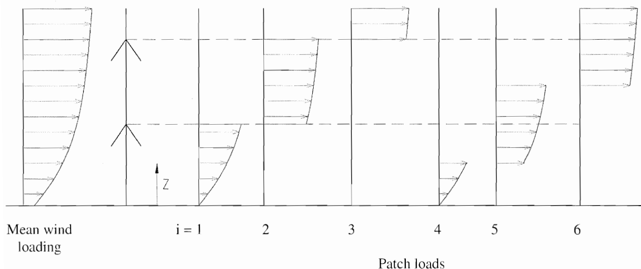
Figure B.4.1 Application of patch loads
