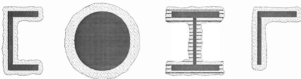
Figure C.1 Ice thickness on structural members
