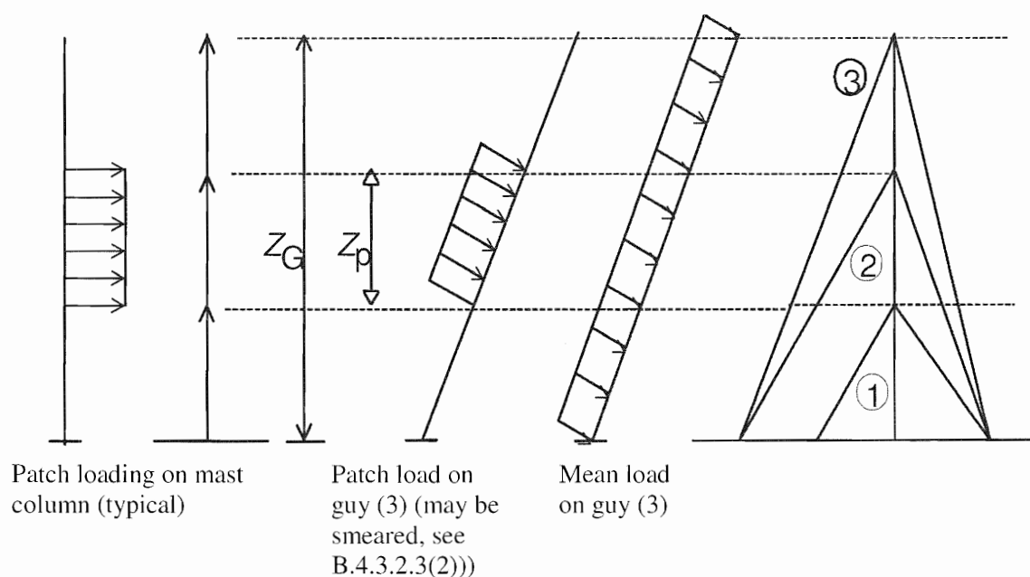
Figure B.4.2 Patch loading on guys
