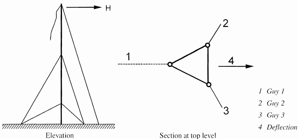
Figure E.1 Guy rupture
