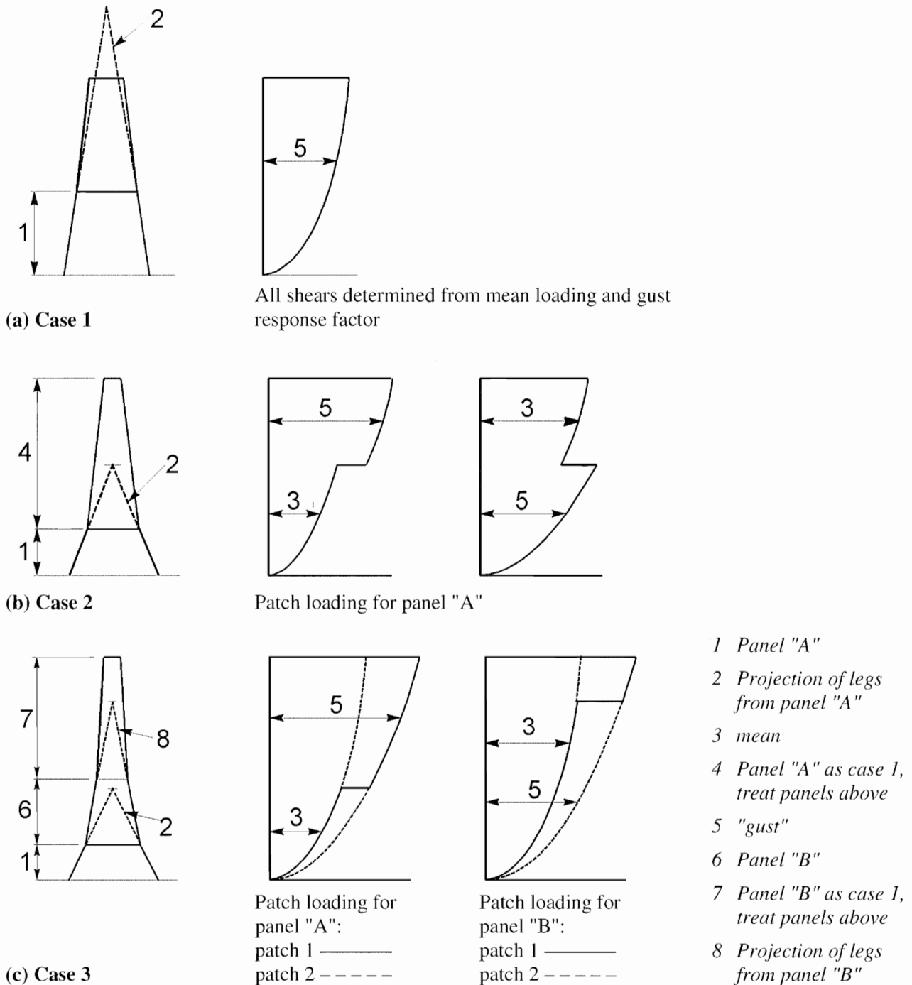
Figure B.3.1 Shear patch loading
