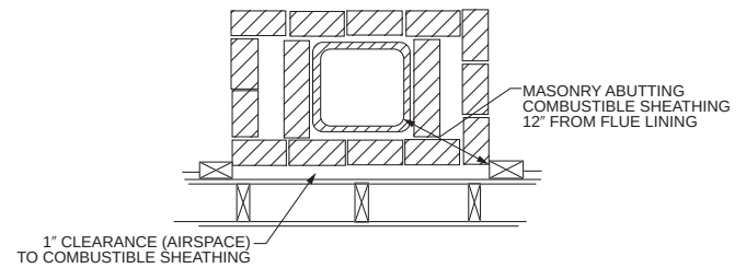
FIGURE 2113.19 ILLUSTRATION OF EXCEPTION THREE CHIMNEY CLEARANCE PROVISION
