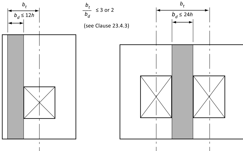
Figure 23.1 Effect of openings on design width, b_d (See Clause 23.4.2.)
