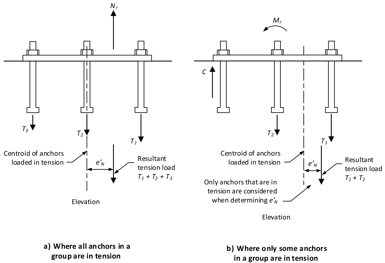
Figure D.9 Definition of dimension e'_N for a group of anchors (See Clause D.6.2.4.)
