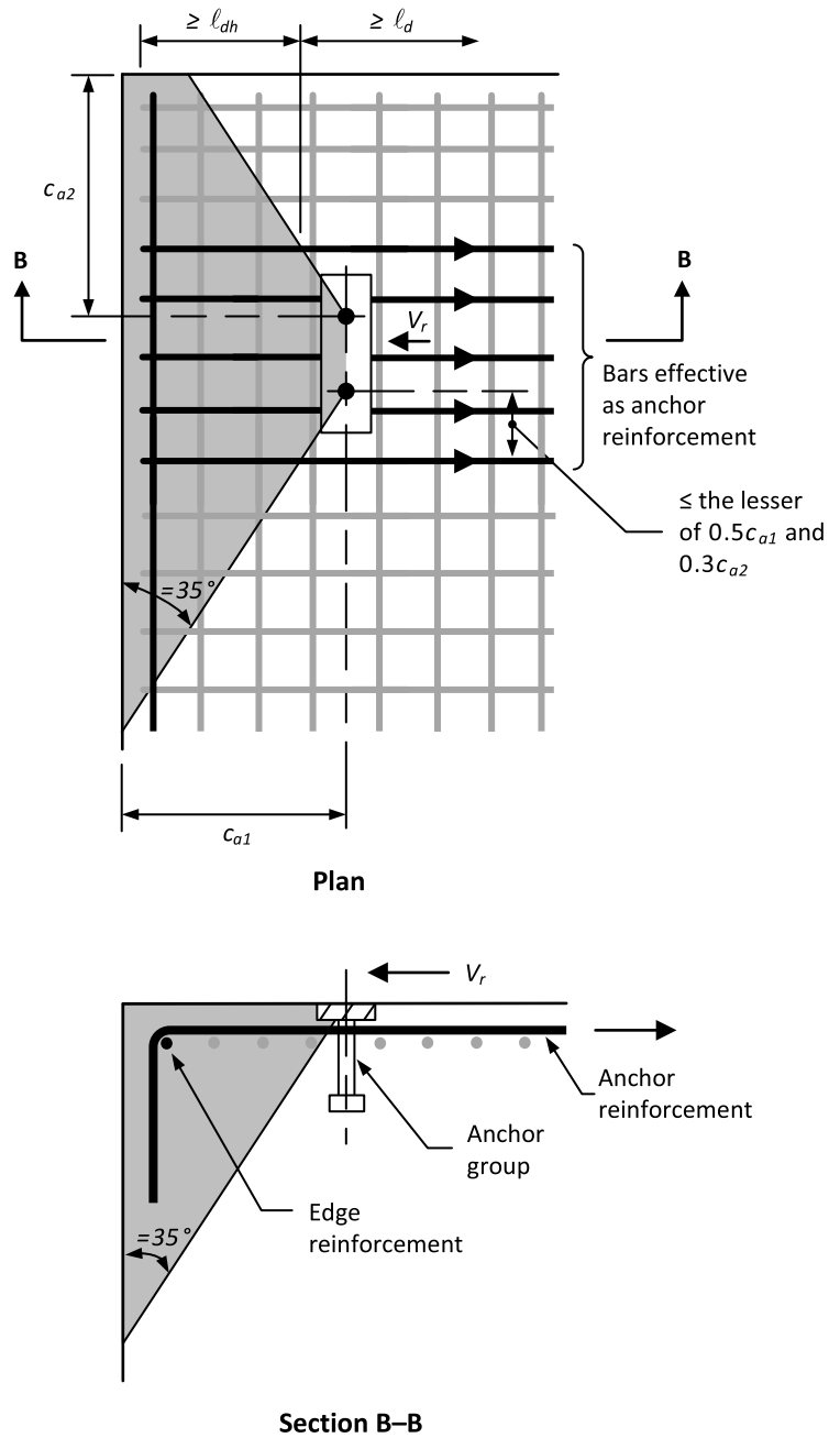
Figure D.17B Edge reinforcement and anchor reinforcement for shear (See Clause D.7.2.9. )
