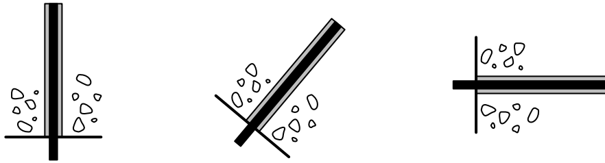
Figure D.2 Possible orientations of horizontal or upwardly inclined anchors (See Clauses D.2 and D.4.3.5.3.)
