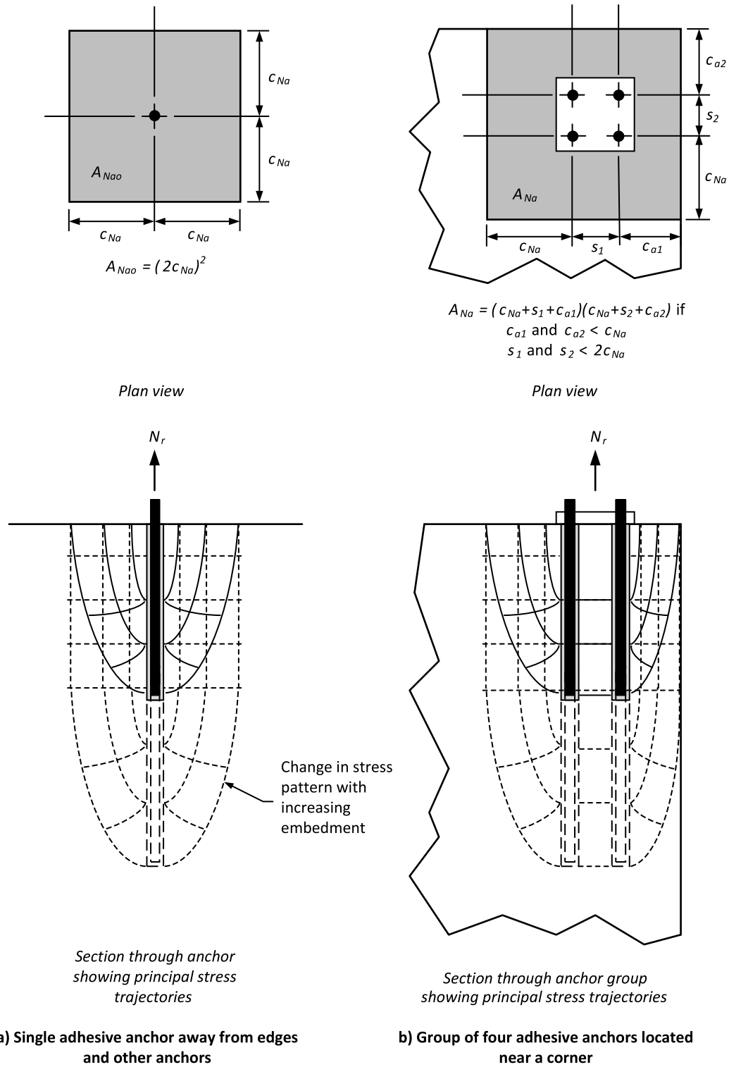
Figure D.11 Calculation of influence areas A_{Na0} and A_{Na} (See Clause D.6.5.1.)
