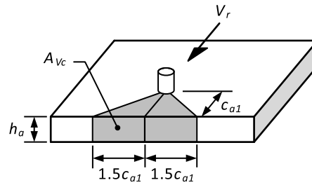
Figure D.13 Projected areas for single anchors and anchor groups (See Clause D.7.2.1.)
