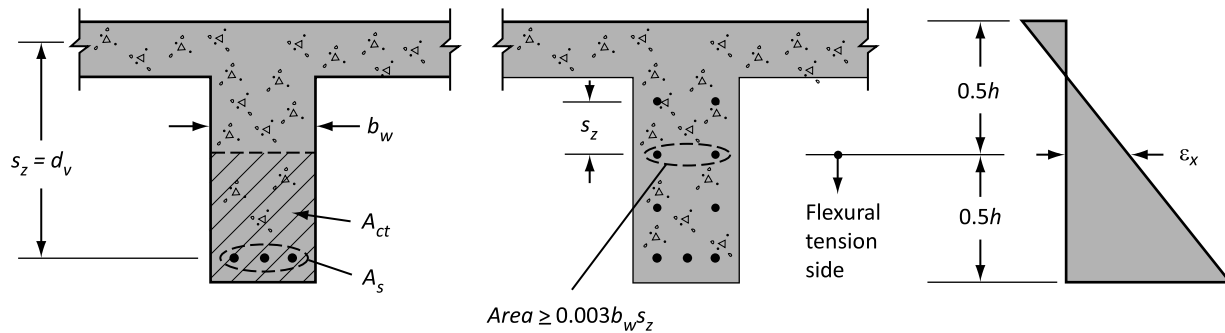
Figure 11.2 Terms in shear design equations (See Clauses 3.2 and 11.3.6.3.)
