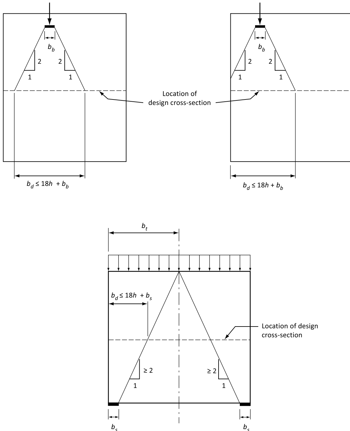
Figure 23.2 Effect of concentrated loads or reactions on design width, b_d (See Clauses 4.1.2, 23.5.1, and 23.5.4.)
