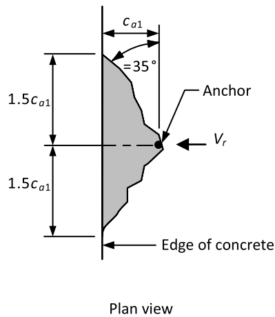
b) Breakout cone for shear
