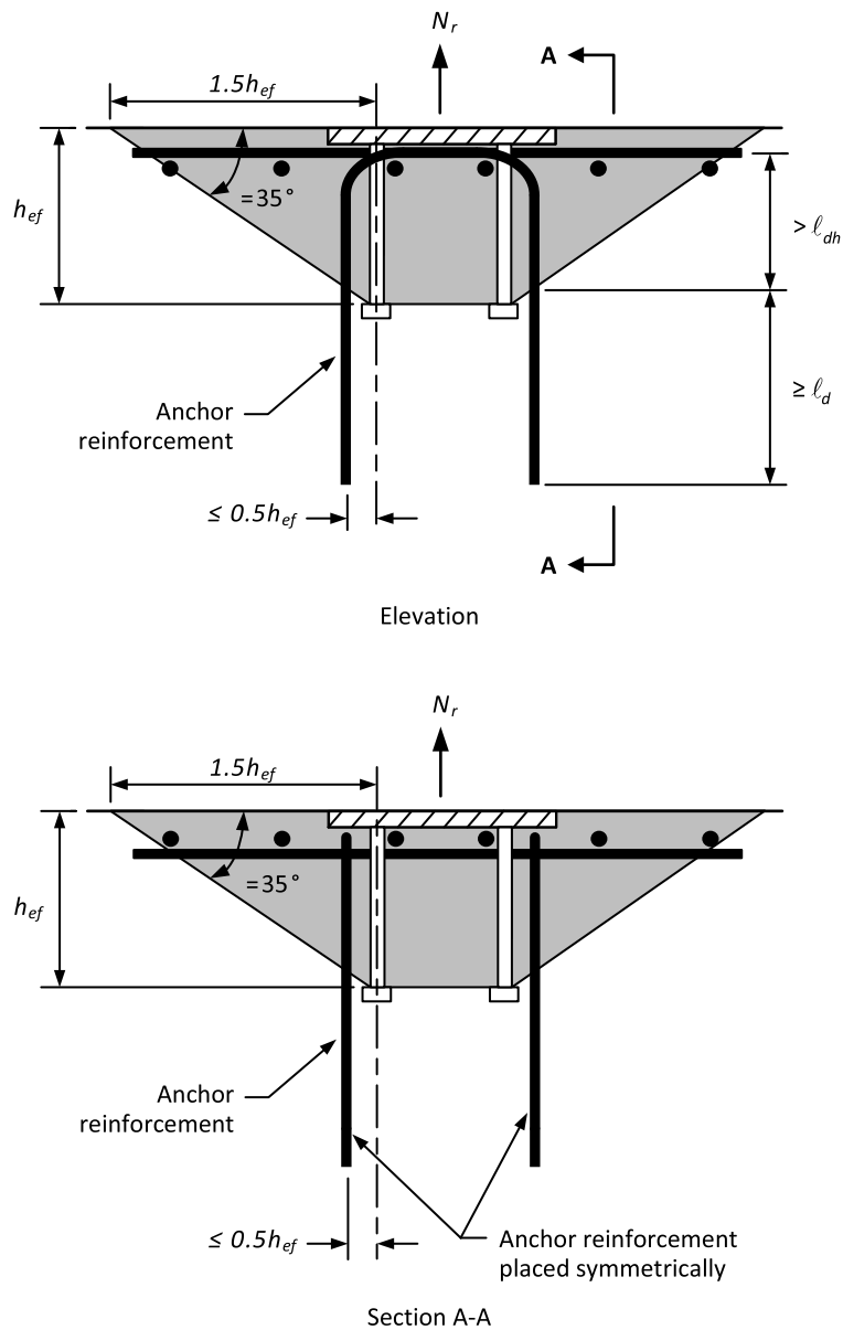
Figure D.10 Anchor reinforcement for tension (See Clause D.6.2.9.)
