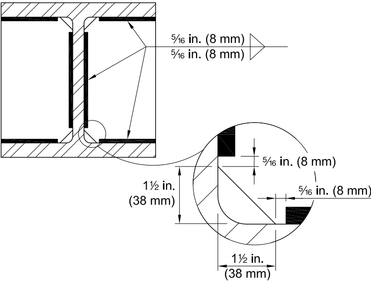
Fig. C-J10.8. Recommended placement of stiffener fillet welds to avoid contact with “k-area.”
